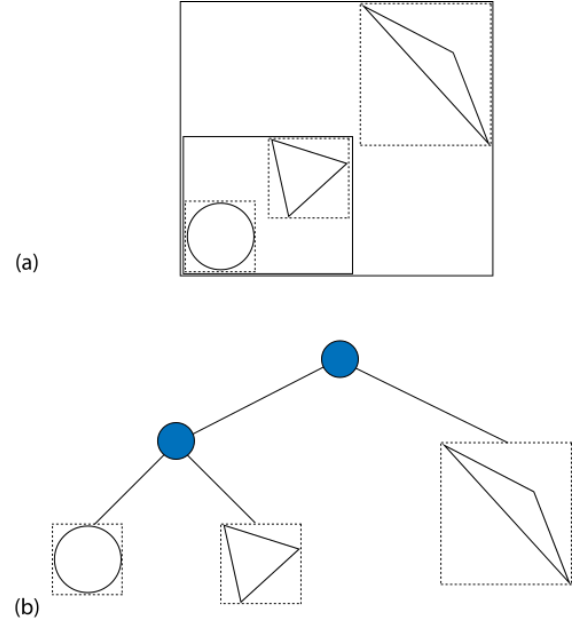
Figure 3: BVH-tree structure. [5]
